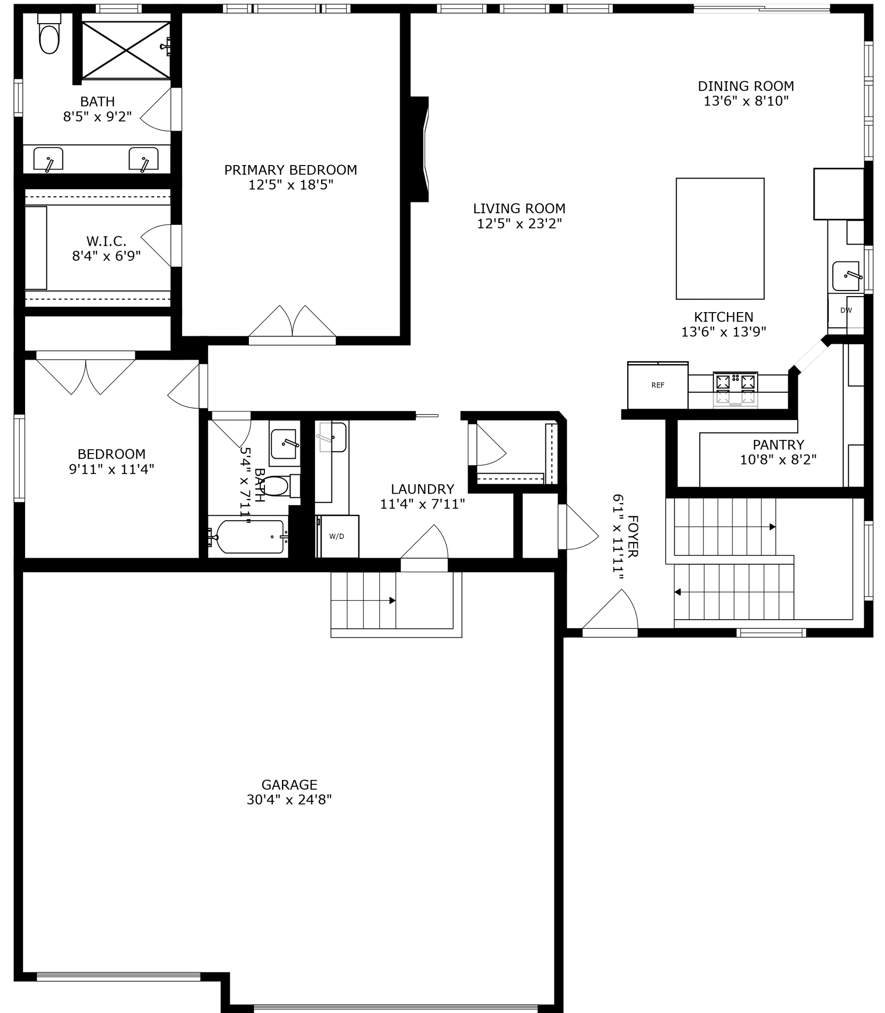
FLOOR 2
