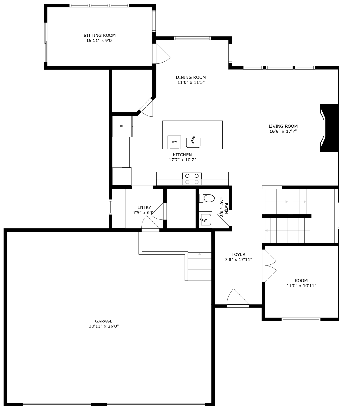
FLOOR 2
